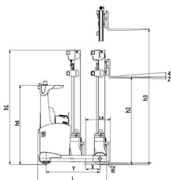
Asst: Right angle stacking aisle width a: Clearance a=200mm
